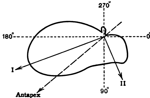
vii. Region XII. ; centre, R.A. 10^{\text{h}} 48^{\text{m}} , Dec. +17^{\circ} .
